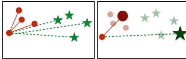
Figure 20: Red circles and green stars represent points of two different classes respectively. There are 48 triplets that can be formed from these instances. Learning a proxy for each class results in only 8 comparisons [15].
