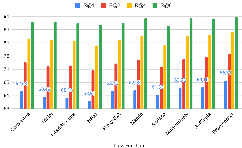
Figure 27: Comparing the retrieval quality of loss functions on CUB200-2011 using ResNet50 with an embedding size of 128.
