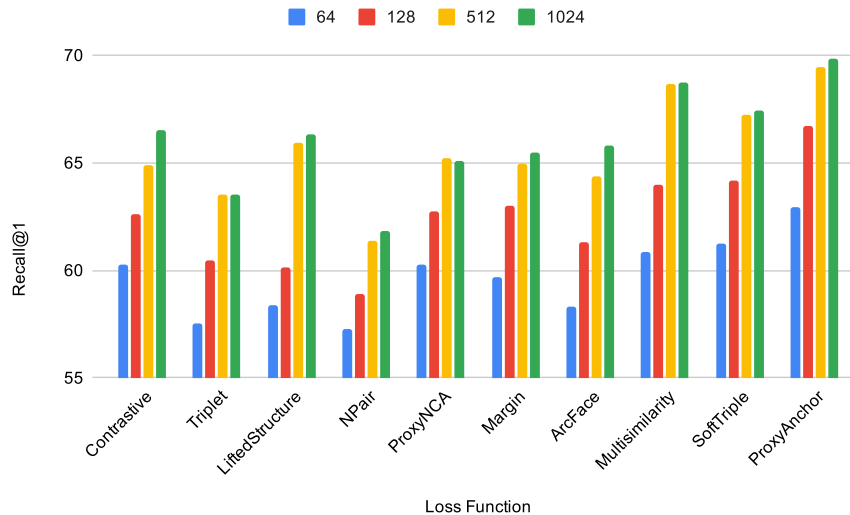
Figure 28: Comparing the retrieval quality of loss functions on CUB200-2011 using ResNet50 with different embedding sizes.
