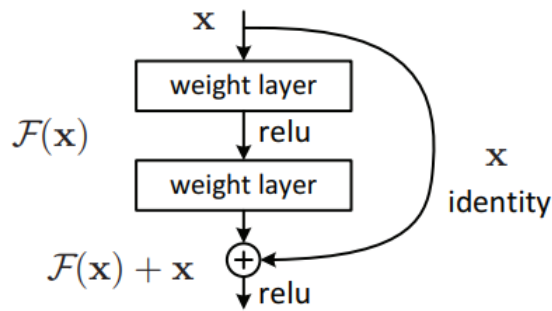
Figure 13: The residual block [12].
