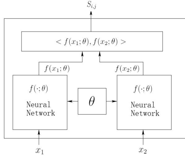
Figure 15: The Siamese Architecture.
