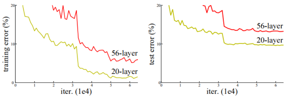
Figure 12: Training and test error of a 20-layer and 56-layer Network. Increasing Network depth leads to worse performance [12].
