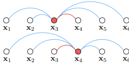
Figure 18: In this illustration with 6 examples, x_3 and x_4 represent a randomly sampled positive pair that independently compares against all other negative pairs in order to mine the hardest one [1].
