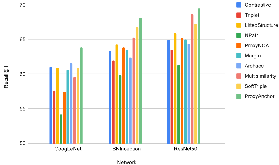
Figure 31: Comparing the discriminative power of Networks. All loss functions use an embedding size of 512.
