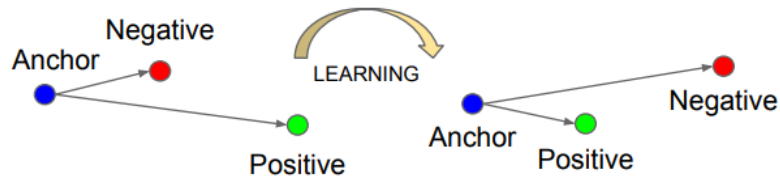
Figure 16: Triplet loss function makes the distance between an anchor and a positive smaller than the distance between this anchor and a negative [13].
