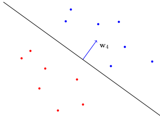
Figure 4: The Perceptron algorithm correctly classifies all data points. The decision boundary w_4 is the weight vector occurred after 4 iterations of the algorithm [4].
