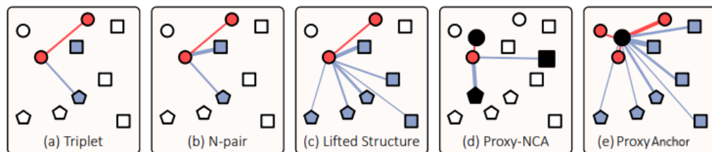
Figure 23: Nodes represent different samples in a batch. Different shapes represent different classes, black nodes represent proxies, red nodes represent positives, blue nodes represent negatives. The associations defined by the losses are expressed by edges and thicker edges get larger gradients. (a) Triplet loss associates each anchor with a positive and a negative without considering their hardness. (b) NPair loss and (c) LiftedStructure loss reflect hardness of data, but do not utilize all data in the batch. (d) ProxyNCA loss cannot exploit data-to-data relations since it associates each data point only with proxies. (e) ProxyAnchor handles entire data in the batch, and associates them with each proxy with consideration of their relative hardness determined by data-to-data relations. See the text for more details [18].
