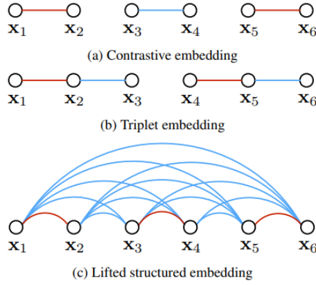
Figure 17: Illustration of a training batch with six samples x_1, \dots, x_6 . Red edges represent positives, while blue edges represent negatives. Contrastive loss function works using separate pairs, thus x_1 and x_2 represent a positive pair, x_3 and x_4 represent a negative pair, etc. Triplet loss function works using separate triplets, thus x_2 represents an anchor that has a positive x_1 and a negative x_3 , etc. In general, a sample x_i of the training batch cannot be used more than once when computing both the Contrastive and Triplet loss function. In contrast, LiftedStructure takes into account all pair wise samples within the batch, thus x_1 and x_2 represent a positive pair, while at the same time x_1 and x_3 represent a negative pair [1].
