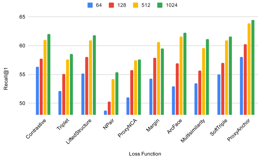
Figure 30: Comparing the retrieval quality of the loss functions on CUB200-2011 using GoogLeNet with different embedding sizes.
