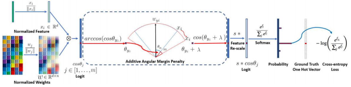
Figure 21: We first normalize the feature x_i and weight w . Then we get the \cos \theta_j logit for each class as w_i^T x_i . We calculate the \arccos \theta_{y_i} and get the angle between the feature x_i and the ground truth weight w_{y_i} . w_j can be seen as a proxy for each class. Then, we add an angular margin penalty \lambda on the target angle \theta_{y_i} . We calculate \cos(\theta_{y_i} + \lambda) and multiply all logits by the feature scale s . The logits finally go through the SoftMax and CrossEntropy. [16]
