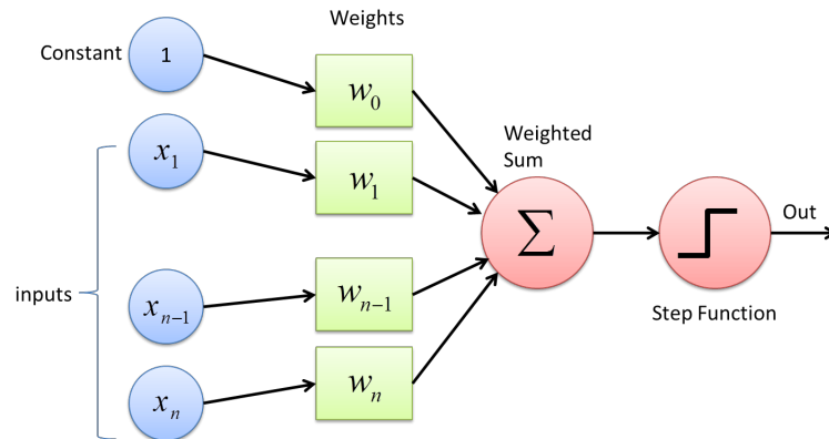
Figure 3: The Perceptron architecture. Apart from the x_1, \dots, x_n , there is also a x_0 = 1 constant term, which is added, so that the weight w_0 plays the role of bias and thus the model takes the generalized form of y = f(x; w, b) = \text{sgn}(w^\top x + b) [3].
