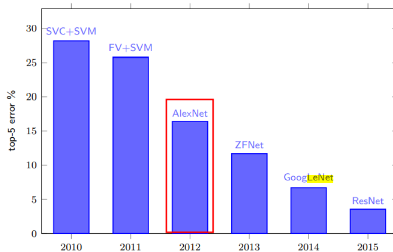
Figure 7: ILSVRC top-5 error% per year in classification task [7].
