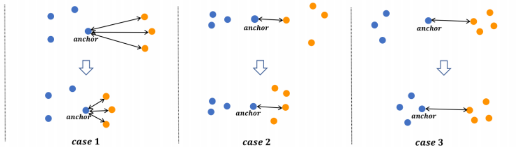
Figure 19: The three types of similarity [14].
