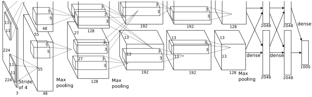
Figure 9: The AlexNet architecture [9].
