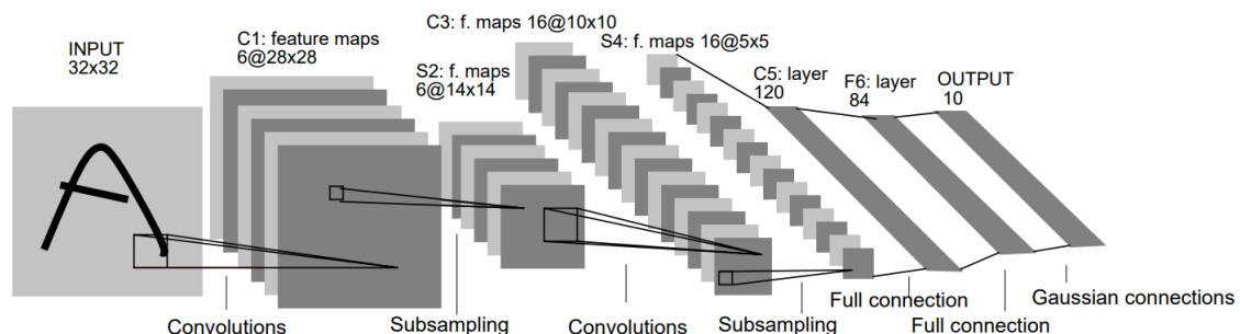
Figure 6: The LeNet architecture [6].
