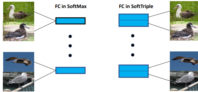
Figure 22: In SoftMax loss, each class has only one corresponding proxy. Samples of the same class will be collapsed to the same proxy no matter their possible variance (pose, color, viewpoint, etc.). In contrast, SoftTriple keeps multiple proxies and thus is more capable of modeling the intra-class variability, as these samples will be assigned to different proxies. [17]
