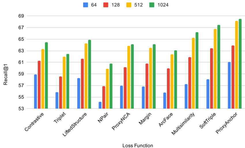
Figure 29: Comparing the retrieval quality of the loss functions on CUB200-2011 using BNInception with different embedding sizes.
