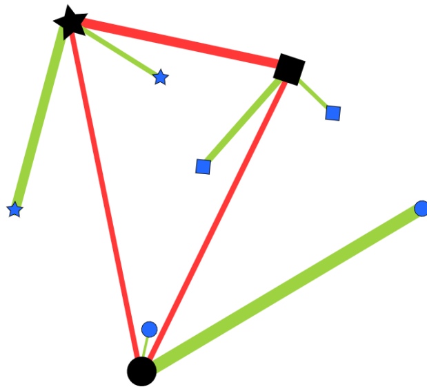
Figure 32: Visualization of the way our loss function works. Different shapes correspond to different classes. Black nodes represent proxies, while blue nodes represent samples. Green edges represent positive associations, while red nodes represent negative associations. Thickness is analogous to gradients that samples or proxies get. For example, let us examine the case of the star class that has two positive samples and two negative proxies. Concerning positives, star class is pulling closer both samples, but with different degrees of strength determined by their relative hardness. The star sample that is further away gets larger gradient than the other one. Exactly the opposite is happening concerning negatives, as the square proxy that is closer gets larger gradient than the circle proxy.
