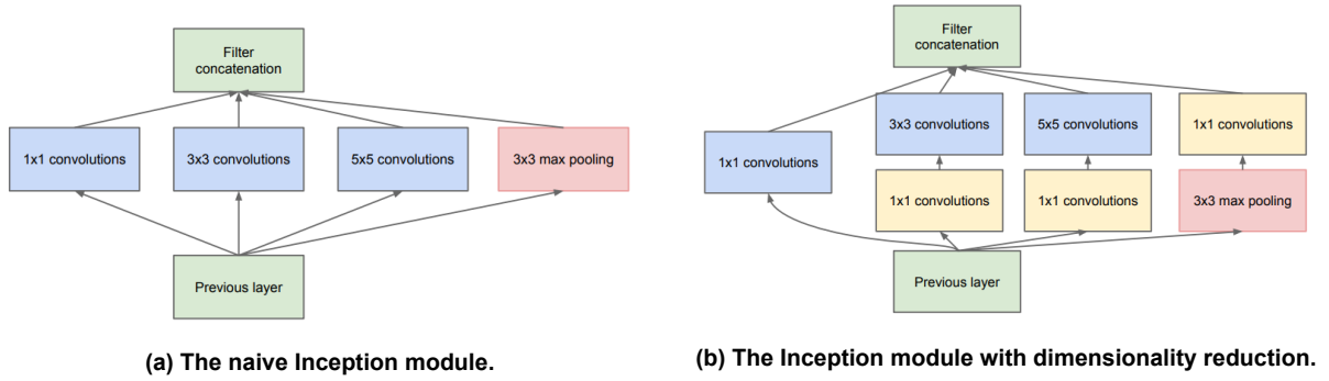
Figure 10: The Inception modules [10].
