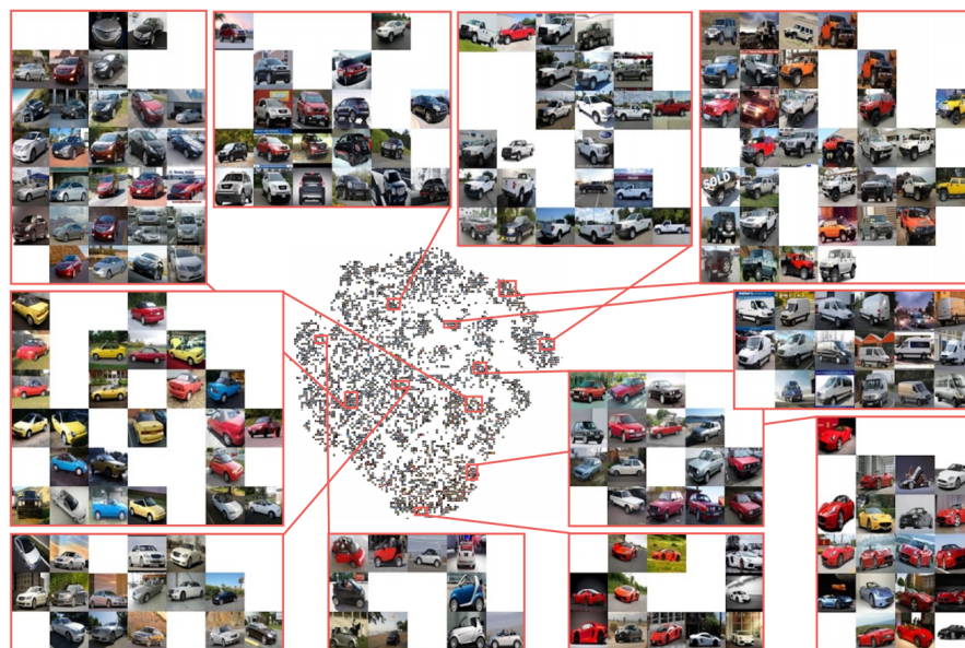
Figure 1: Visualization of the embedding space on the test split of CARS196 using the LiftedStructure loss [1].
