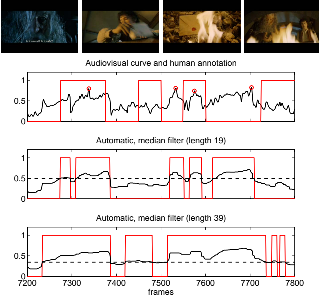
Fig. 2. Main keyframes and human vs. automatic saliency annotations for median-filtered audiovisual curves.
