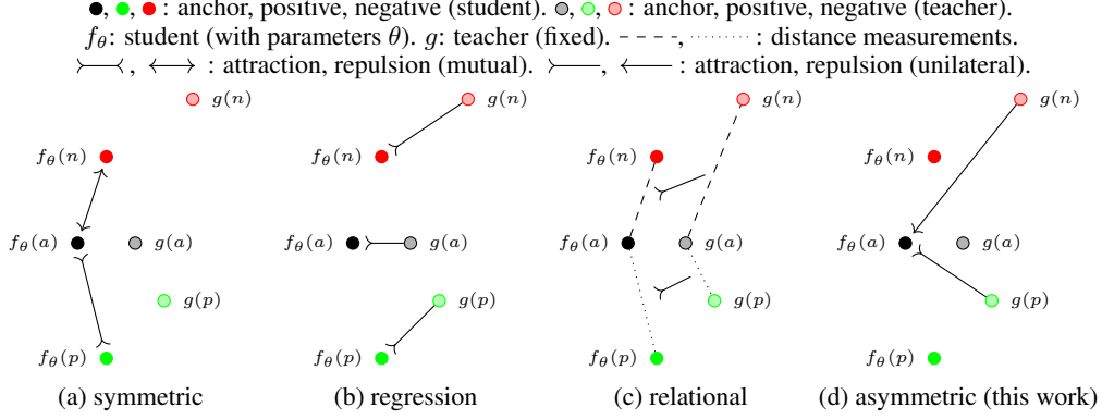
Figure 1: Metric learning and knowledge transfer. (a) Symmetric : Positive (negative) pairs of examples mutually attracted (repulsed) in student space; teacher not used. (b) Regression (absolute ML+KD [81]): Examples in student space attracted to corresponding examples in teacher space; labels not used. (c) Relational (relative ML+KD [81] or distance-wise RKD [47]): Distances encouraged to be the same in both spaces; labels not used. (d) Asymmetric (this work): Anchors in student space attracted to (repulsed from) positives (negatives) in teacher space; both labels and teacher used.
