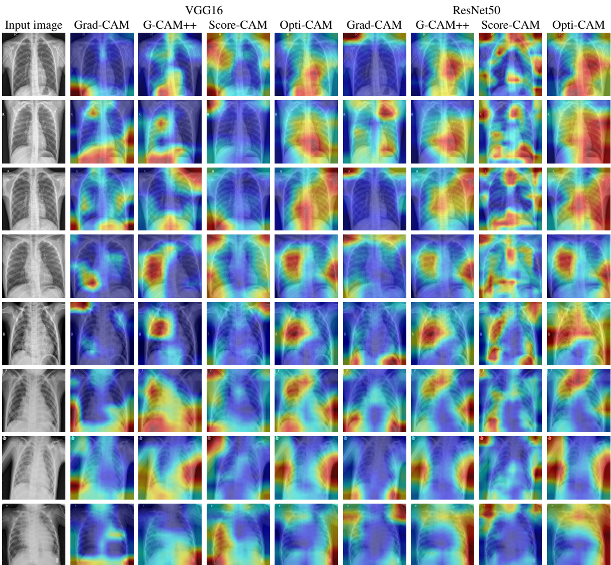
Fig. A8. Saliency maps obtained from Chest X-ray images.
