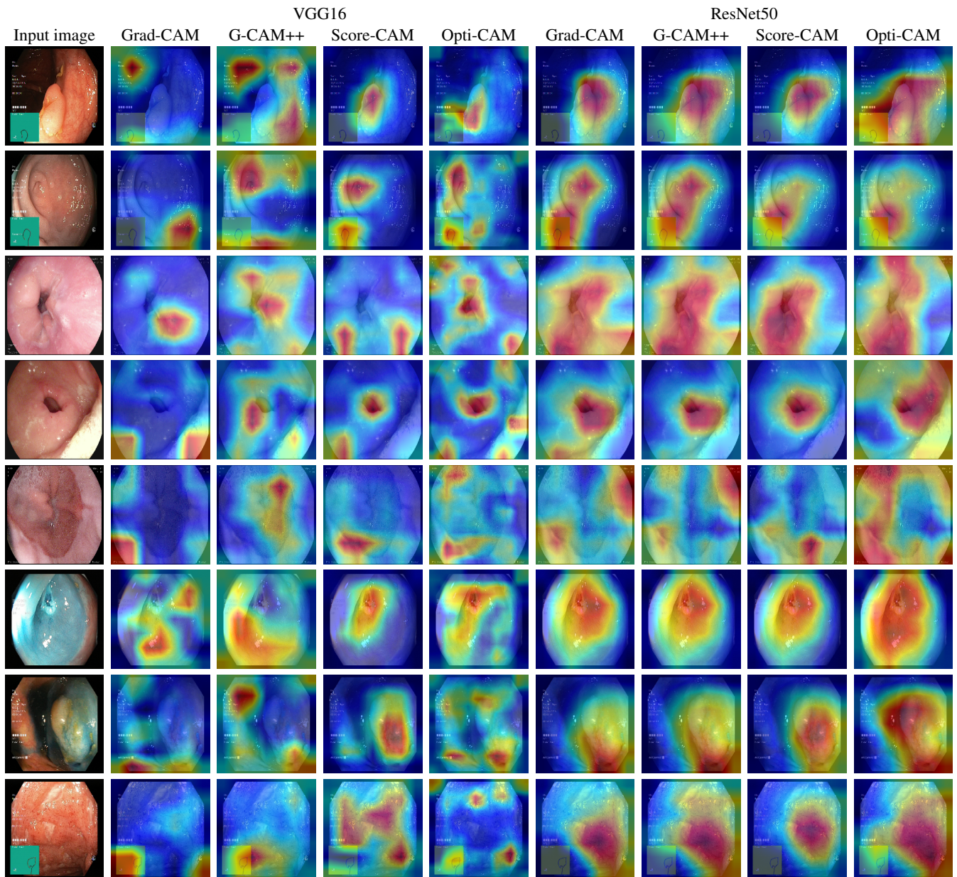
Fig. A9. Saliency maps obtained for KVASIR images.
