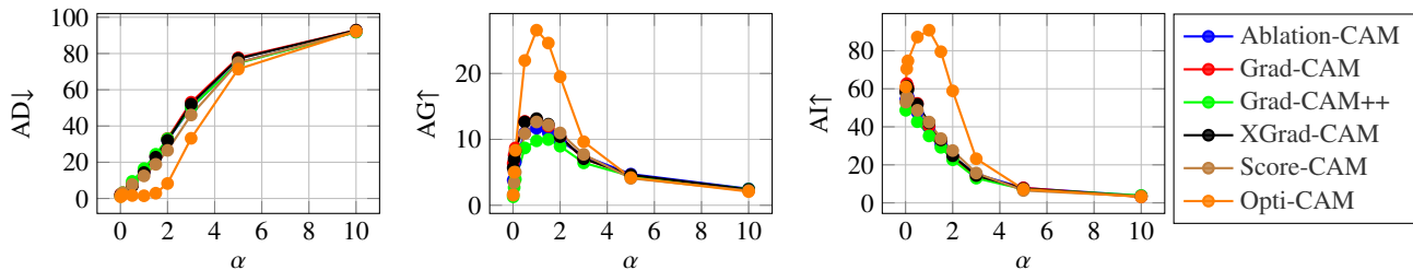
Fig. A4. Effect of selectivity (raising element-wise to exponent \alpha ) of saliency maps on classification performance. AD/AI: average drop/increase (11); AG: average gain (ours); \downarrow / \uparrow : lower / higher is better.
