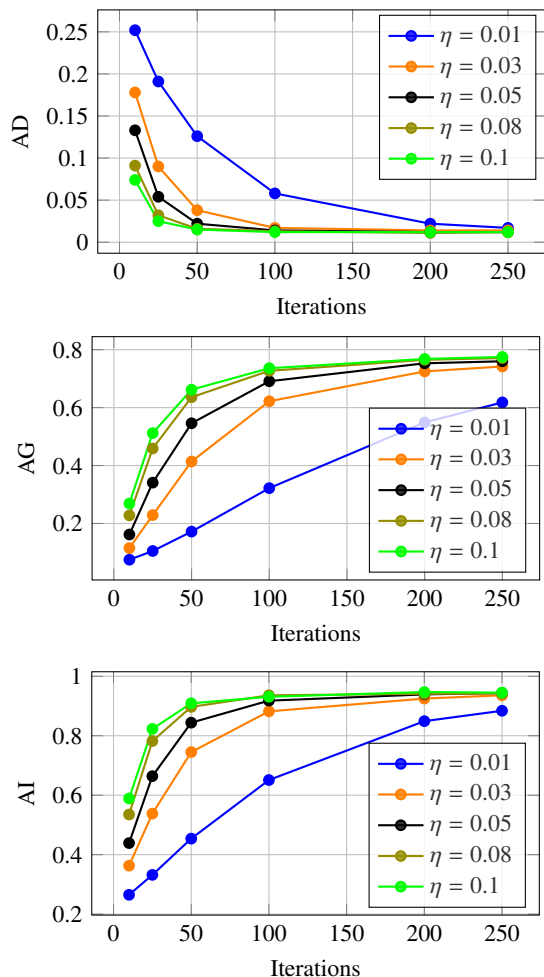
Fig. A5. Classification metrics vs. number of iterations for different learning rates, using VGG-16 on 1000 images of ImageNet. AD/AI: average drop/increase (11); AG: average gain (ours); \downarrow / \uparrow : lower / higher is better.
