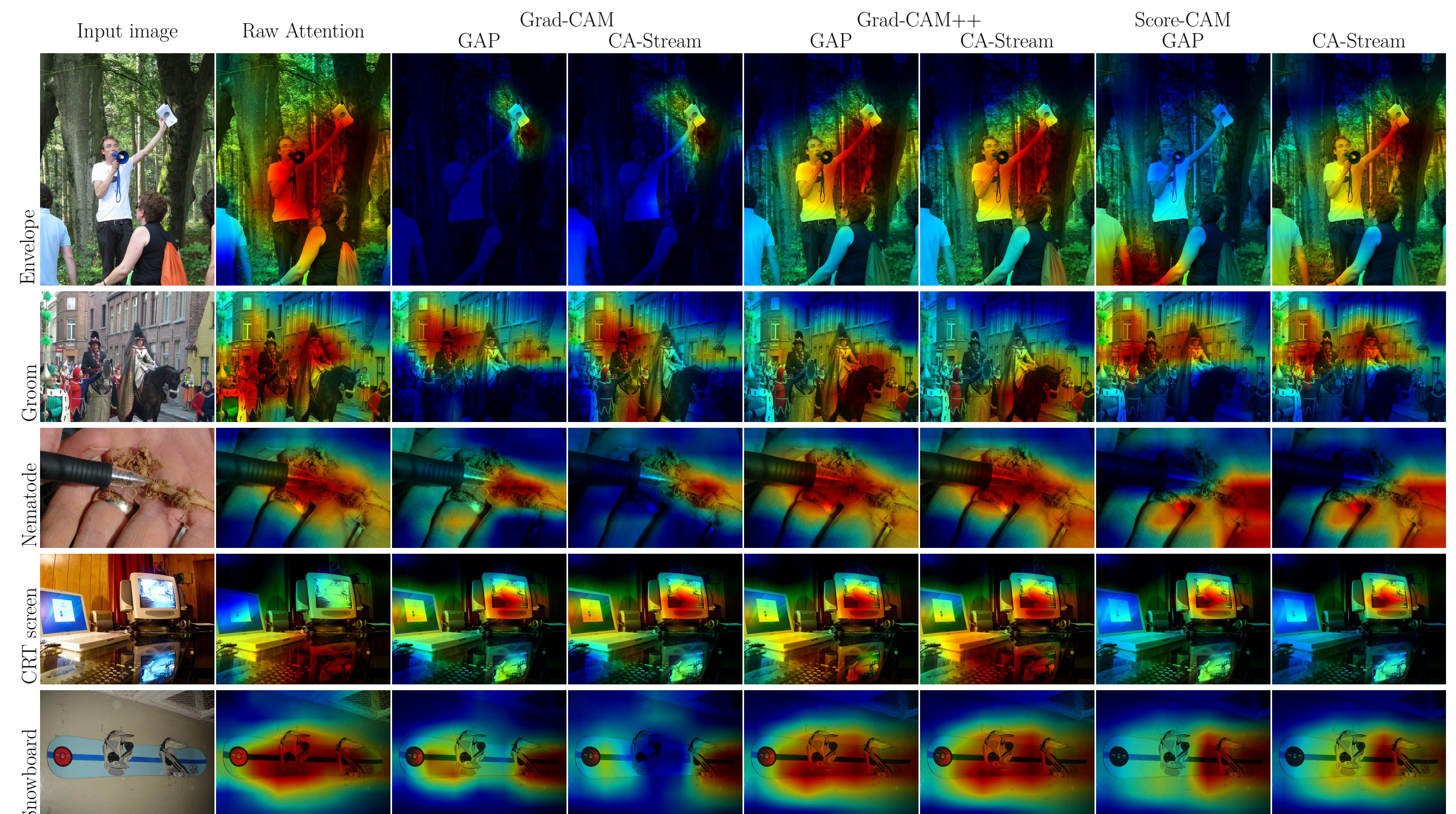
Figure 2: Comparison of saliency maps generated by different CAM-based methods, using GAP and our CA-Stream, on ImageNet images. The raw attention is the one used for pooling by CA-Stream.
