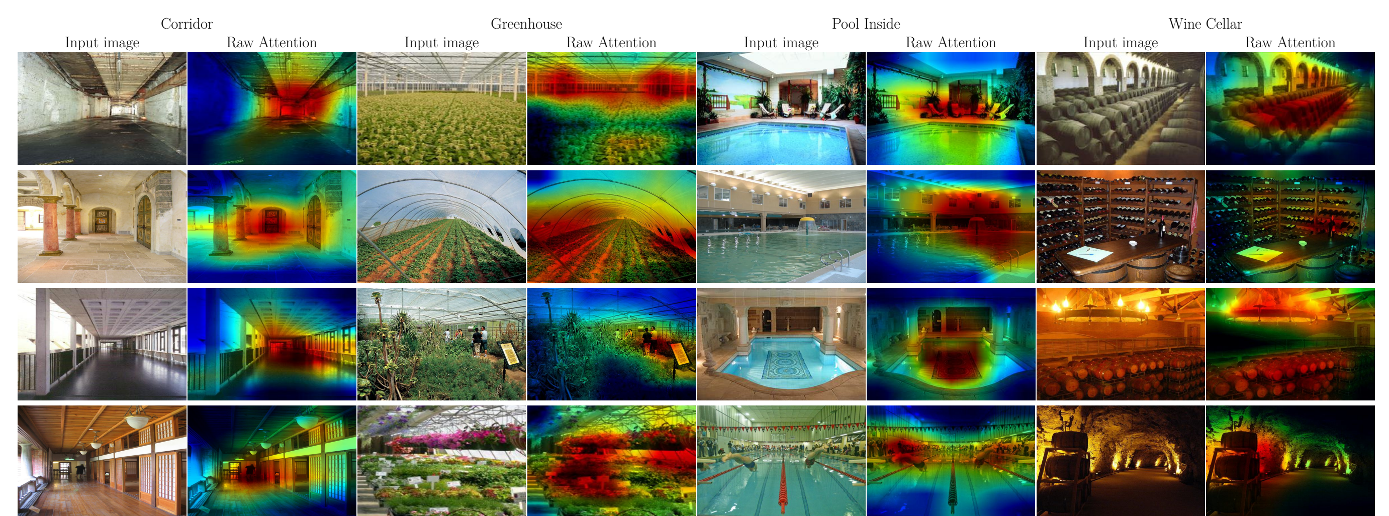
Figure 3: Raw attention maps obtained from our CA-Stream on images of the MIT 67 Scenes dataset [3] on classes that do not exist in ImageNet. The network sees them at inference for the first time.
