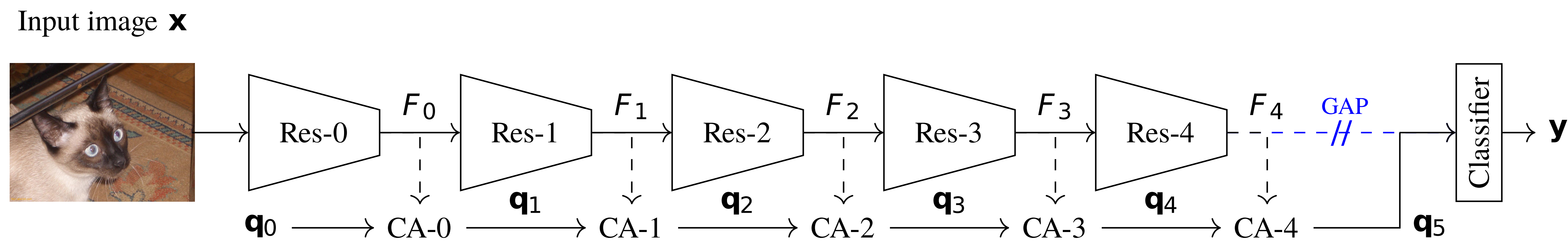
Figure 1: Cross-Attention Stream applied to ResNet-based architectures. During inference, we replace global average pooling (GAP) with our attention-based pooling mechanism, learned with a stream running in parallel to f
